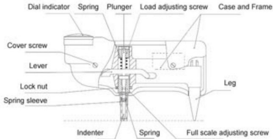
Fig.1 Structure of Barcol Impressor
